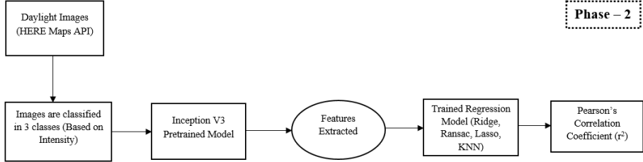
FIG. 3. Phase 2 for the training, regression and prediction of poverty.
