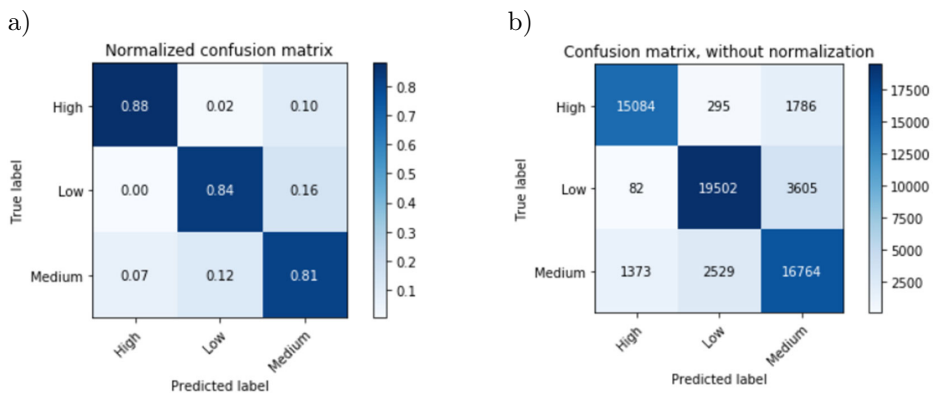
FIG. 18. Confusion matrices with standardization (a) and without standardization (b).
