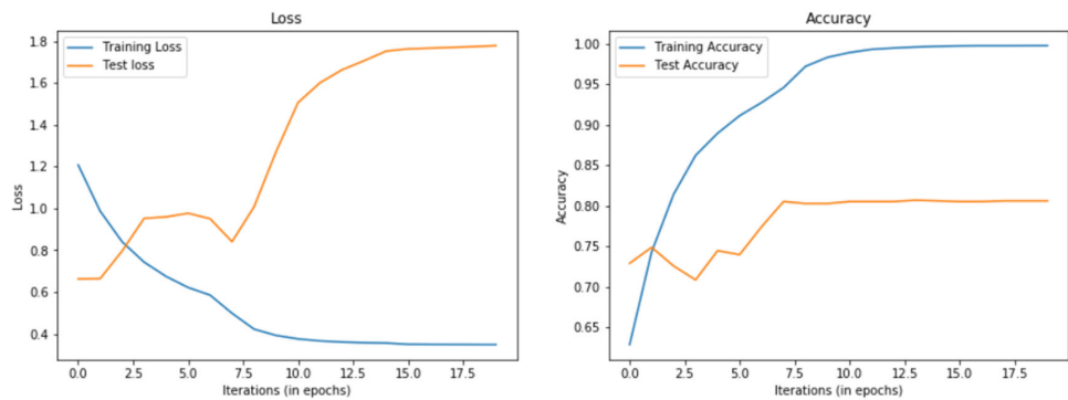
FIG. 4. Iteration vs. loss and accuracy graph.
